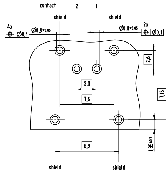
A PCB layout
