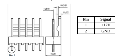
Connector (CN3) : For System Fan Connector. (+12V) Molex 22-27-2021 or equivalent.
