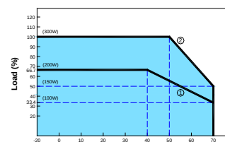
■ De-rating Curve A1 (Load VS Ambient)
