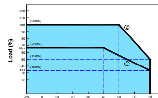
■ De-rating Curve A1 (Load VS Ambient)
