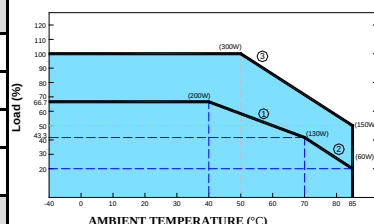
■ De-rating Curve A1 (Load VS Ambient)
